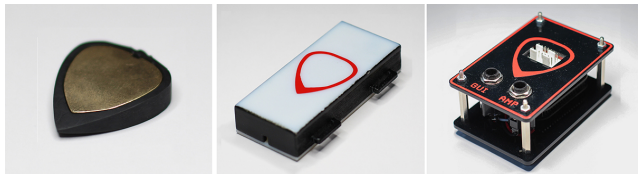
Figure 2: The Magpick; wrist-mounted preamp; stompbox
